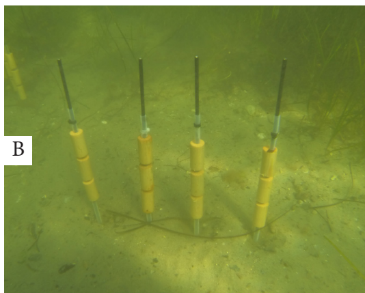
Figure 16. Dr Charlotte Björdal from the University of Gothenburg preparing modern wood samples (A). On each kebab there are two sets of samples that are buried within the sediment and one set of samples exposed to the open seawater as a negative control. (B). Photos National Museum of Denmark.
