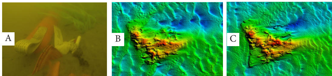
Figure 31. After only 6 days the mats have caught some sediment. Photo RCE Maritime Programme (A). Monitoring from 2012, without the seagrass (B). Monitoring from July 2013 shows that the effects of the mats are already clearly visible (left bottom corner) (C). Image by Periplus Archeomare B.V.
