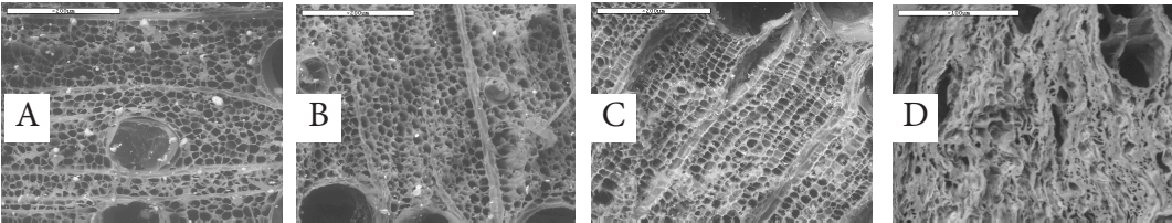
Figure 25. SEM of the non-frozen wood (A). SEM of the wood covered with gyttja (B). SEM of the wood covered with sand and water (C). SEM of ovendried wood (D). Photos National Museum of Denmark.
